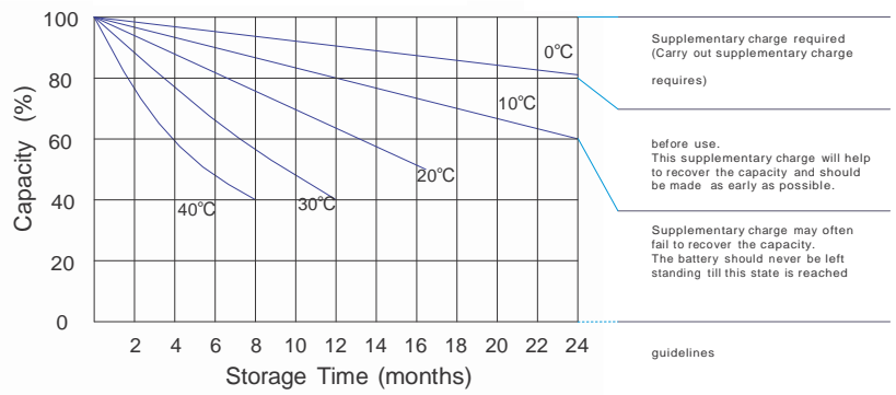
Storage characteristics
